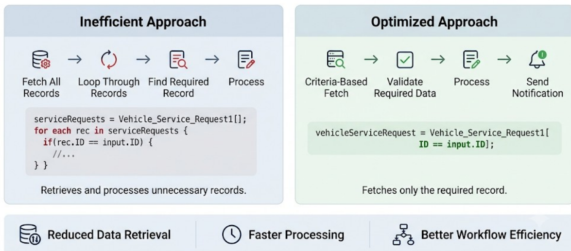
Figure 2: Inefficient and Optimized Approaches (Conceptual Diagram)
