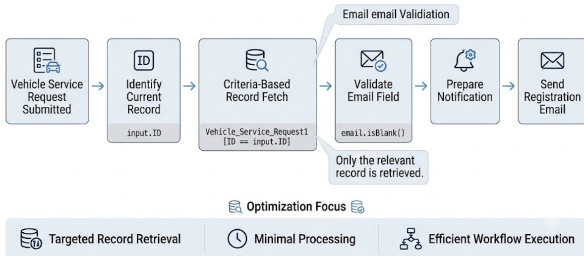
Figure 4: Optimized Vehicle Service Request Workflow (Conceptual Diagram)
